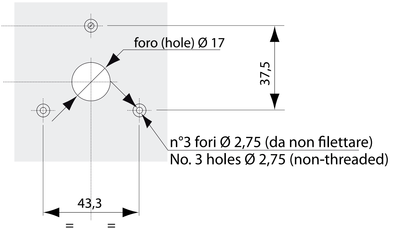
drilling template
