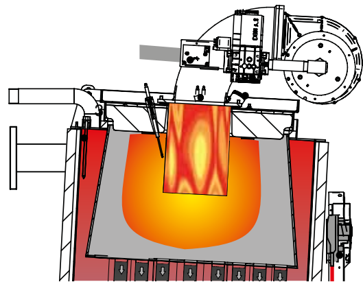
ARES PRO 230 ÷ 600 Combustion chamber
